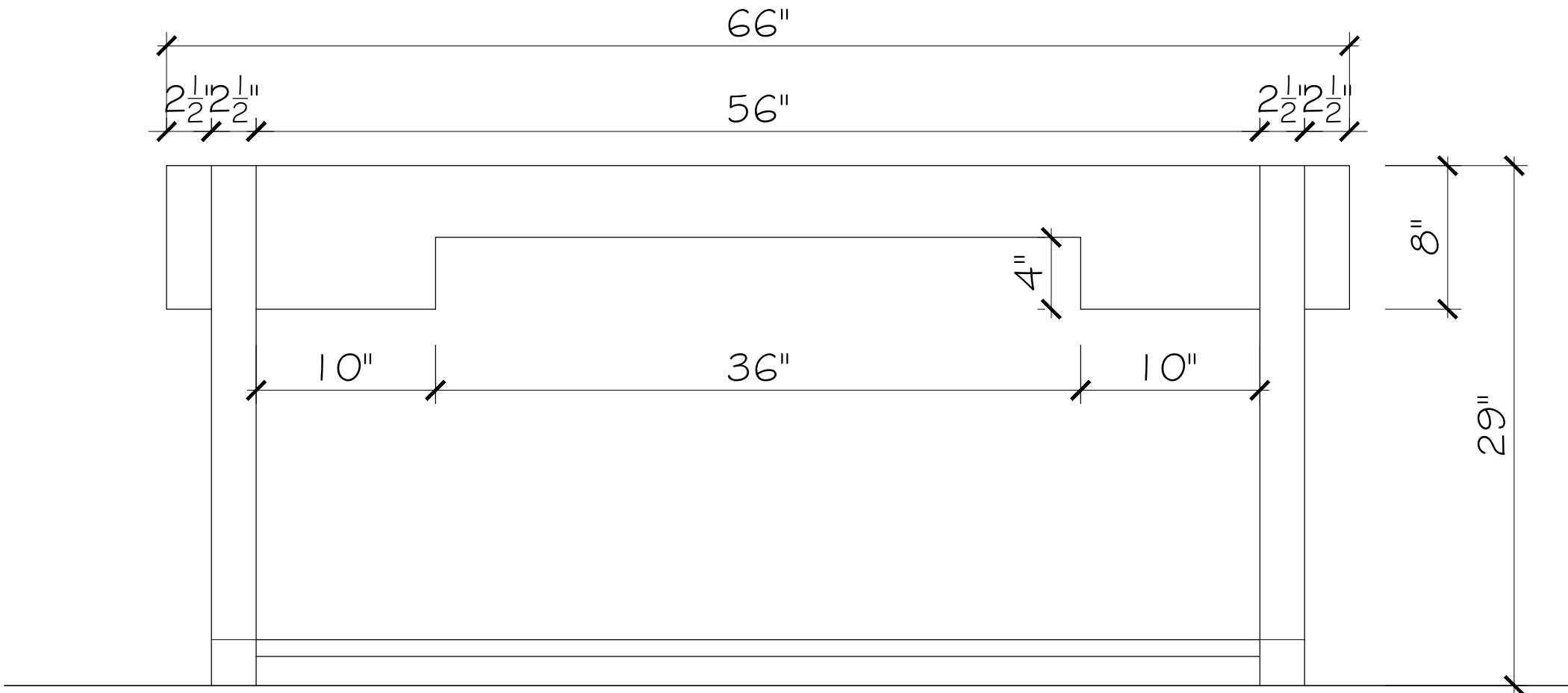
3 ELEVATION BACK VIEW SCALE: 3/4"= 1'-0" RECEPTION DESK
