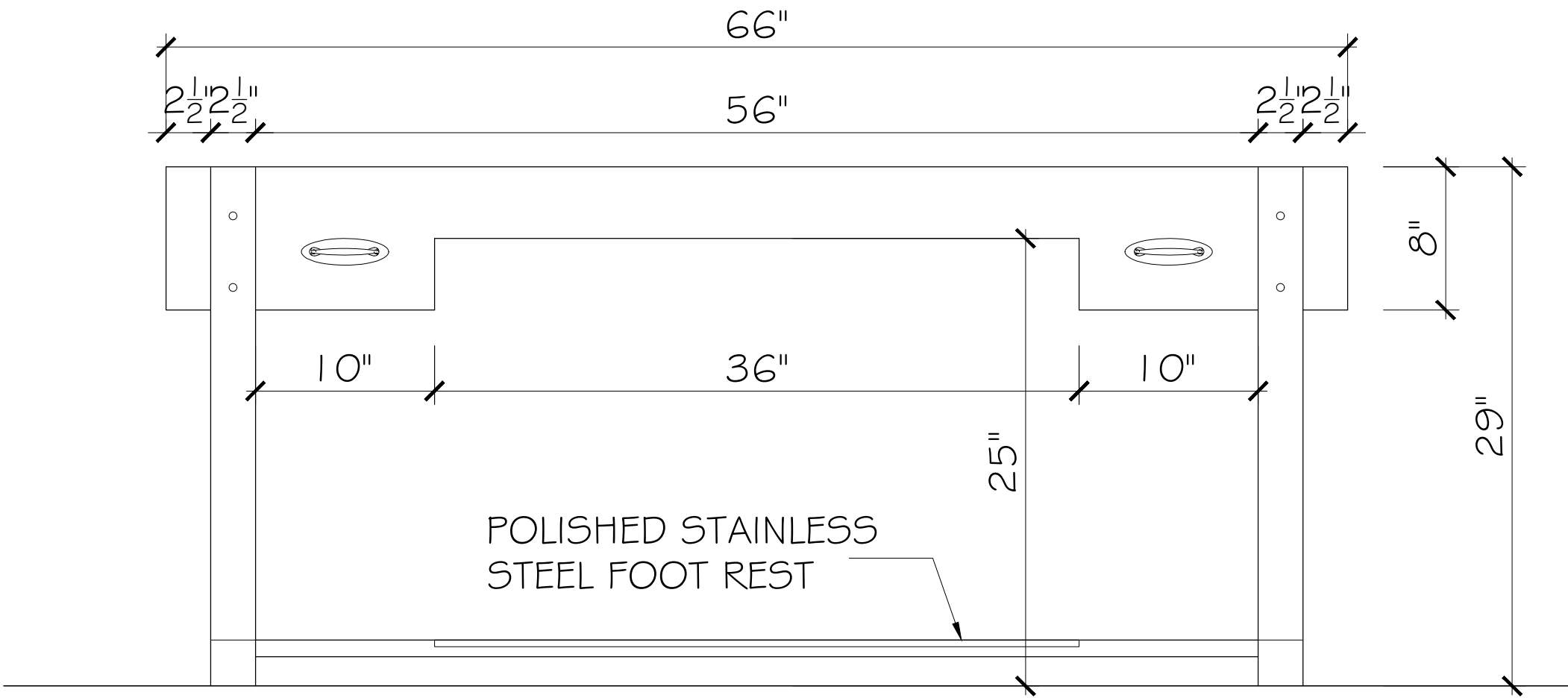
1 ELEVATION FRONT VIEW SCALE: 3/4"= 1'-0" RECEPTION DESK
