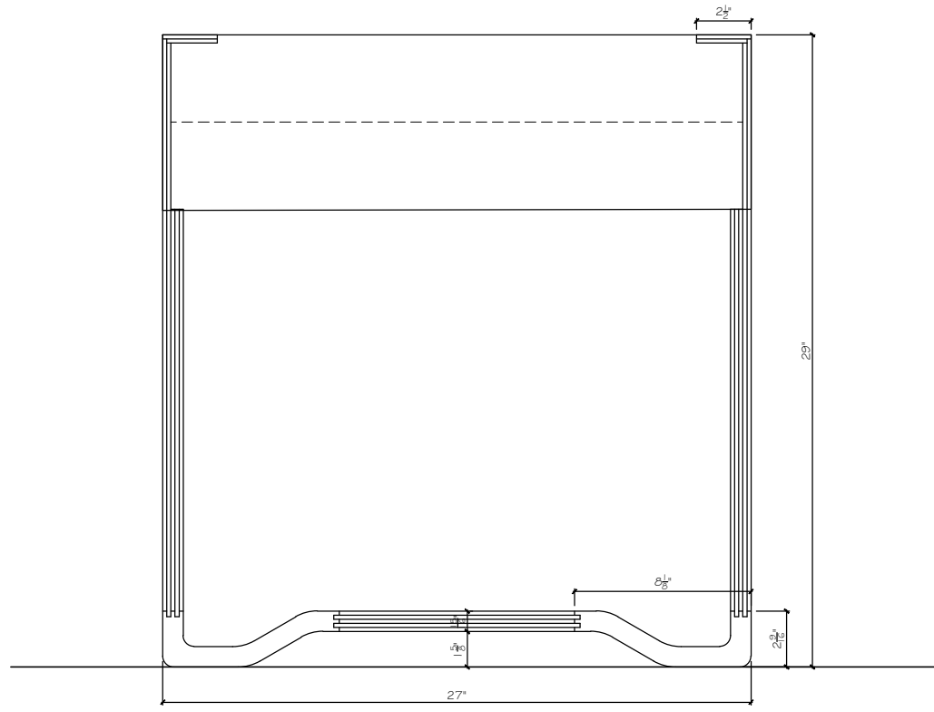
2 ELEVATION SIDE VIEW SCALE: 3/4"= 1'-0" RECEPTION DESK
